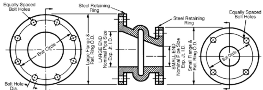
Eccentric Taper
