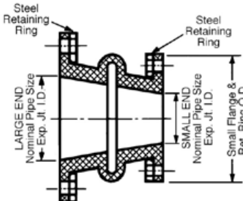
Concentric Taper
